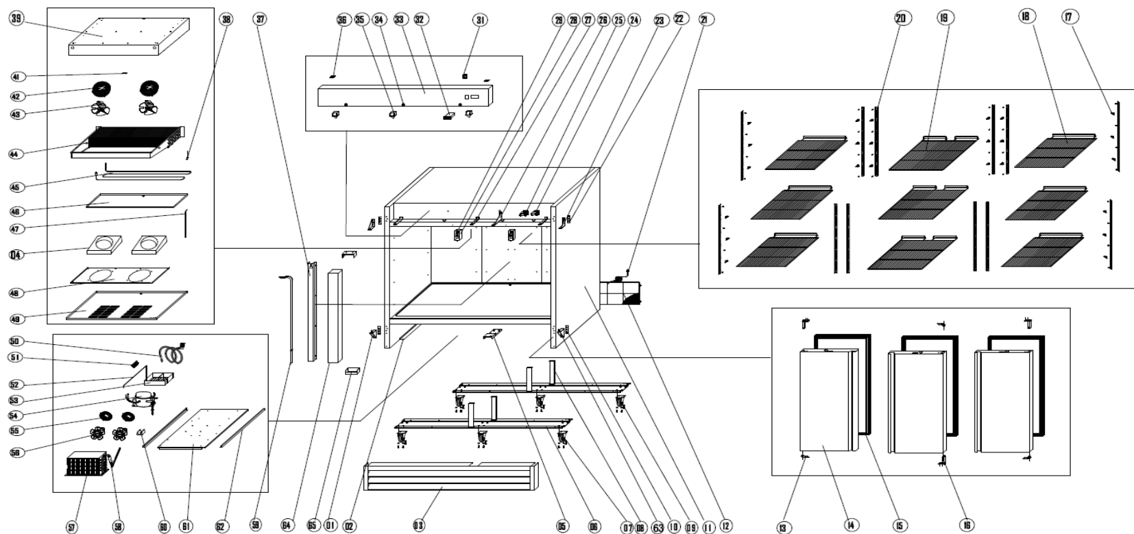
EXPLODE OF KCHRI81R3DF (R404a Version)
